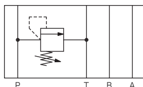
溢流阀 C1M-3F(K)
