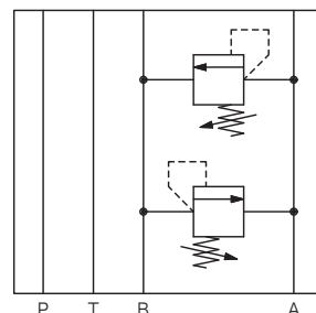
双溢流阀 C2M-3C(K)
